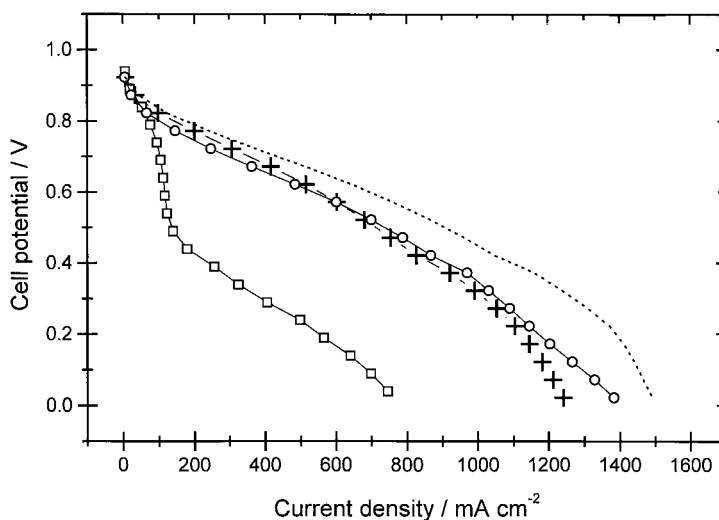
Fig. 1. Polarization curves in H 2 + 100 ppm CO of Pt Black (□), Pt 0.5 Ru 0.5 Black (○) and the ball-milled catalyst Pt 0.5 Ru 0.5 (Al) 4 (+). Polarization curve of Pt 0.5 Ru 0.5 Black in H 2 (- - -) is also shown.
